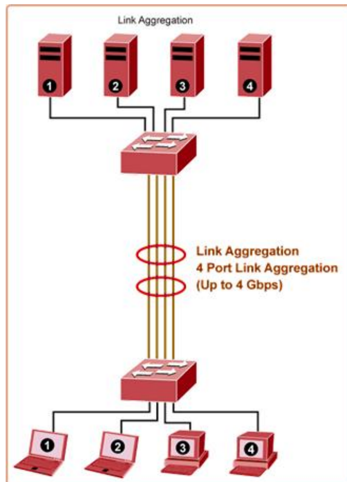
Figure 4-3-23 Link Aggregation
